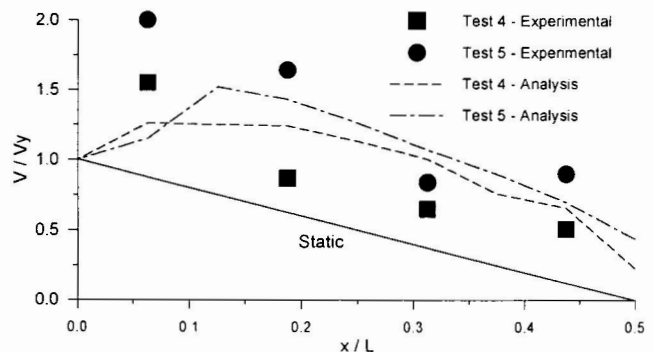
Fig. 6 Shear forces in the diaphragm (Tests #4 & #5).
