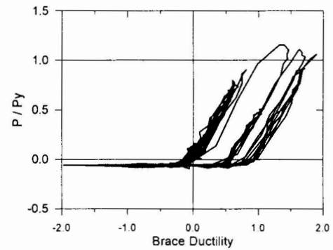
Fig. 5 Brace hysteresis (Test #4).
