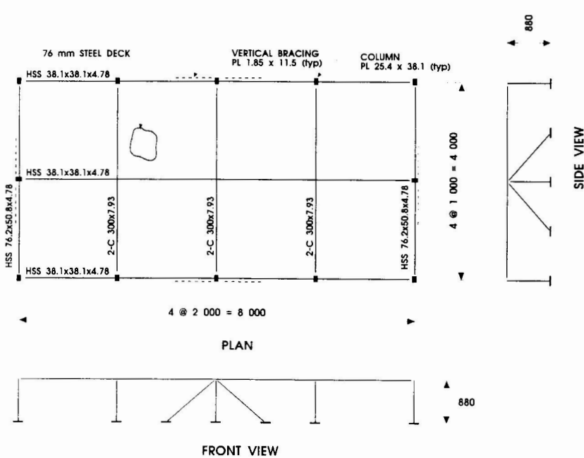
Fig. 3 Building model.
