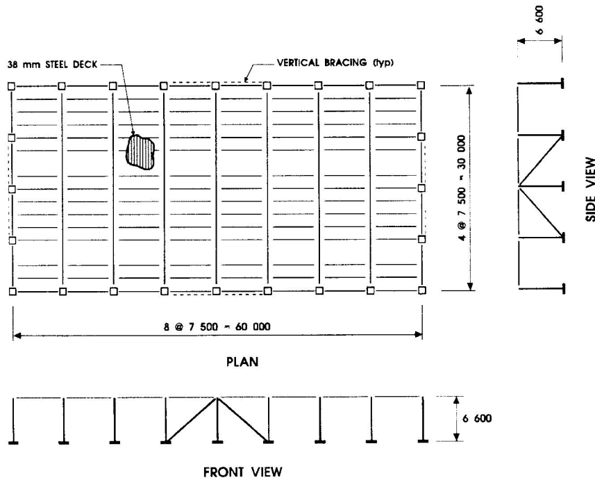
Fig. 2 Prototype building.
