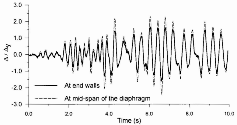
Fig. 4 Time history of relative roof displacements (Test #4).
